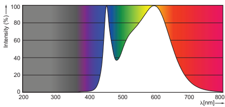
LED tube 1500 mm 22 W /840 C
